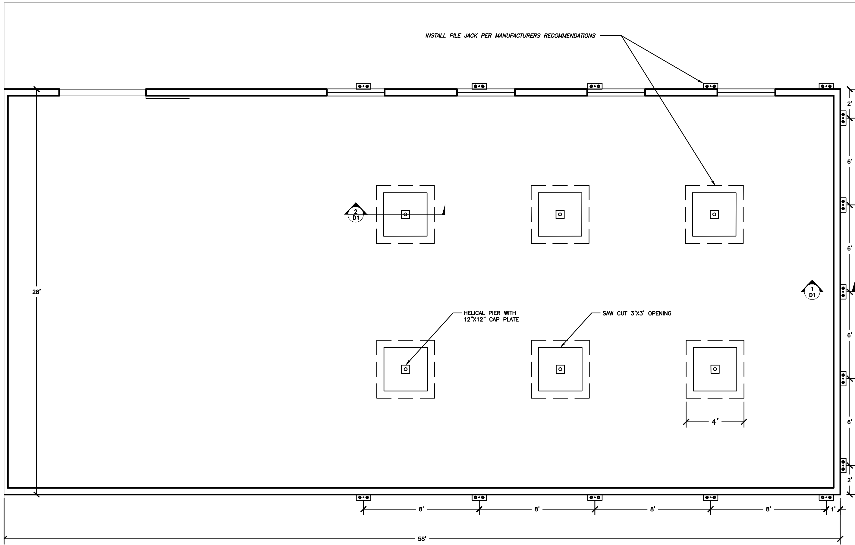
1 FOUNDATION PLAN 1/4" = 1' - 0"
