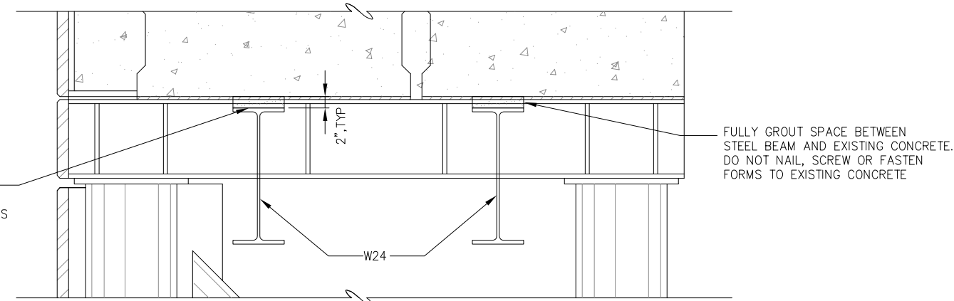
C BEAM TO CONCRETE PANEL GROUTING
