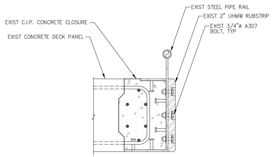
D SECTION AT SIDE CURB (FOR REFERENCE ONLY)
