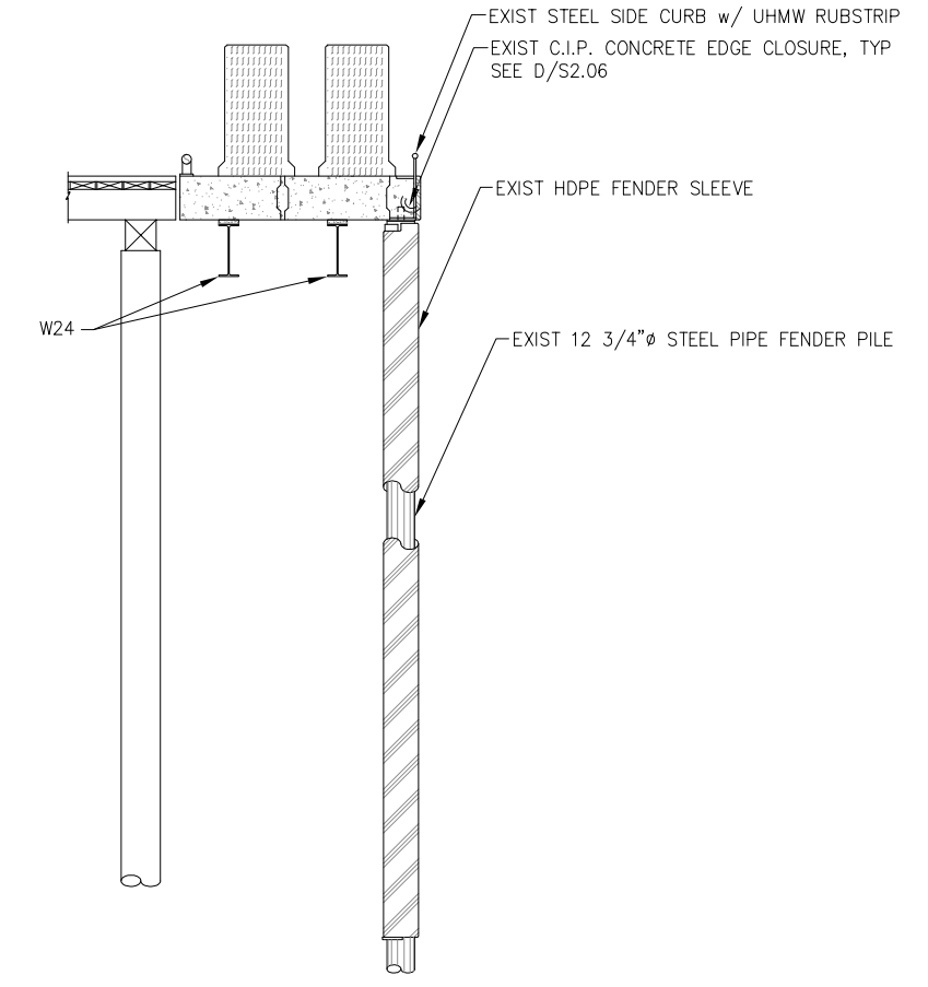
B SECTION AT INTERMEDIATE FENDER PILE
