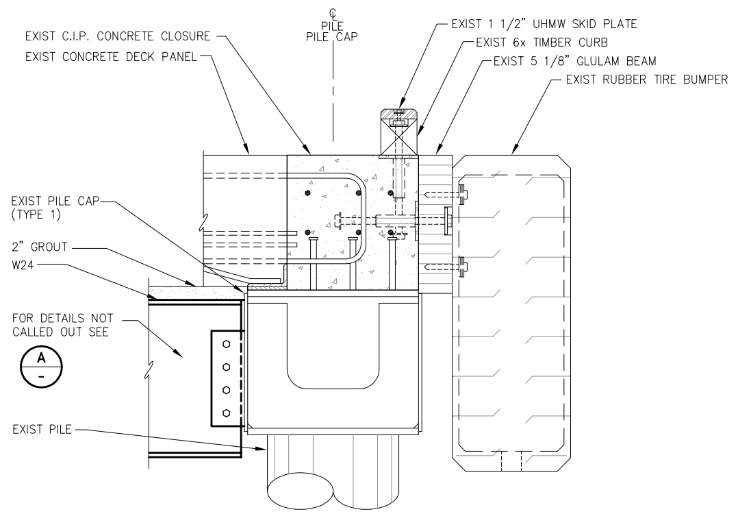
E SECTION AT END CURB
