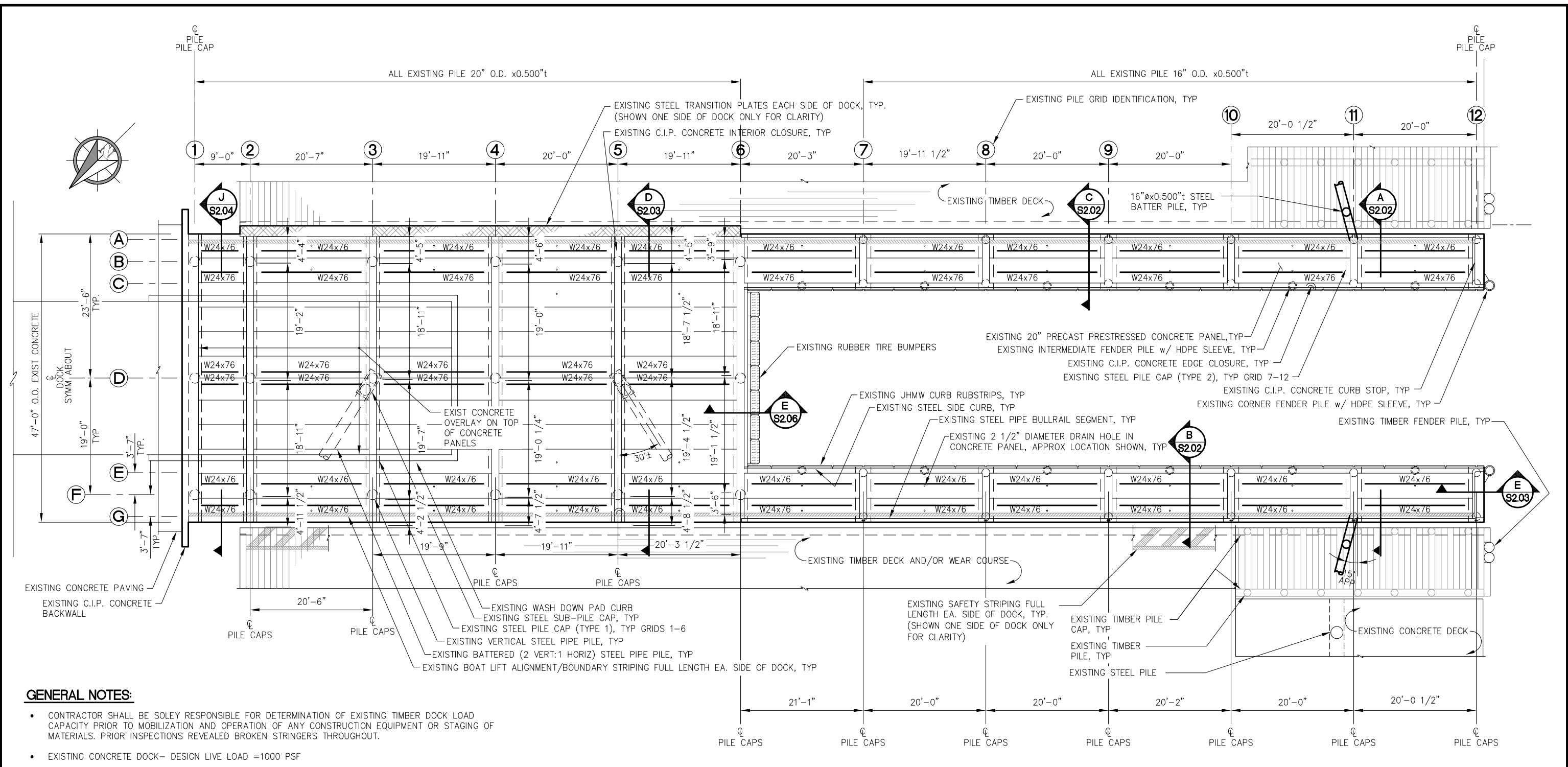
1 DOCK PLAN
