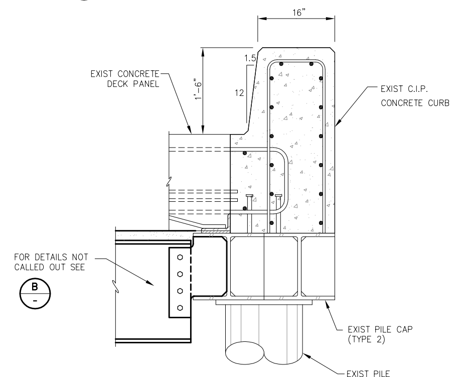
F SECTION AT C.I.P. CURB STOP
