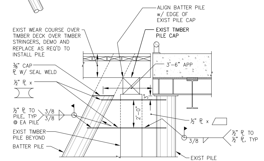
D BATTER PILE CONNECTION DETAIL
