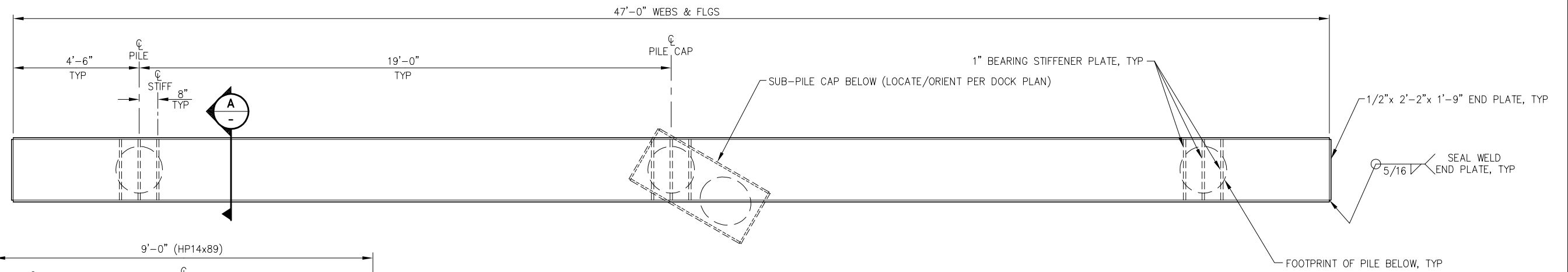
EXISTING PILE CAP TYPE 1 - PLAN (6 TOTAL)
