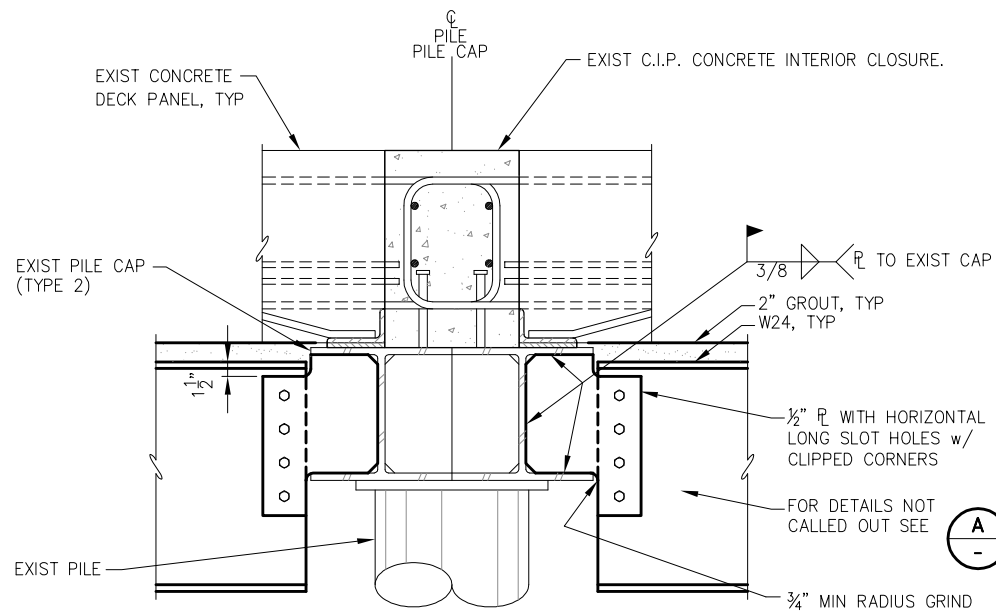
B SECTION AT EXISTING INTERIOR CLOSURE (PILE CAP TYPE 2)
