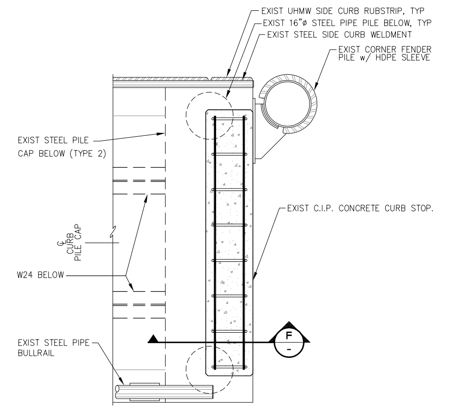
C EXIST C.I.P. CURB STOP - PLAN
