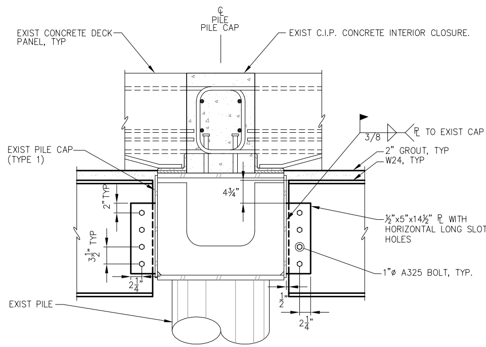
A SECTION AT EXISTING INTERIOR CLOSURE (PILE CAP TYPE 1)
