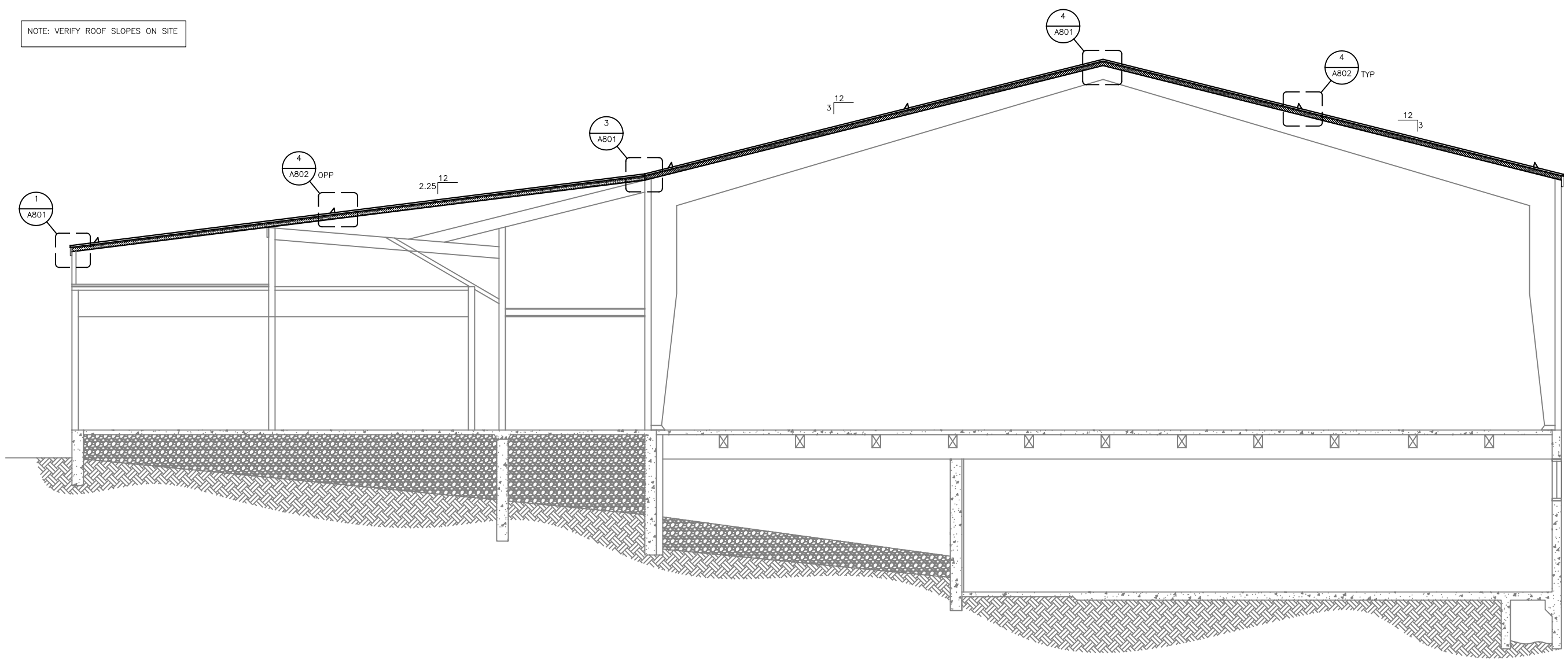
1 BUILDING SECTION
