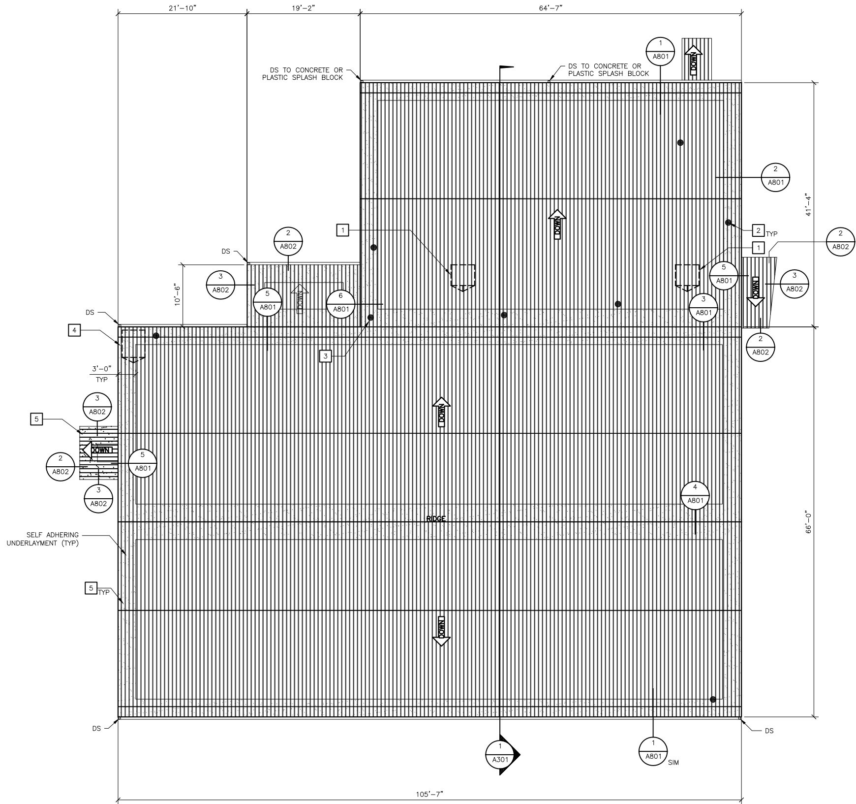
1 ROOF PLAN
