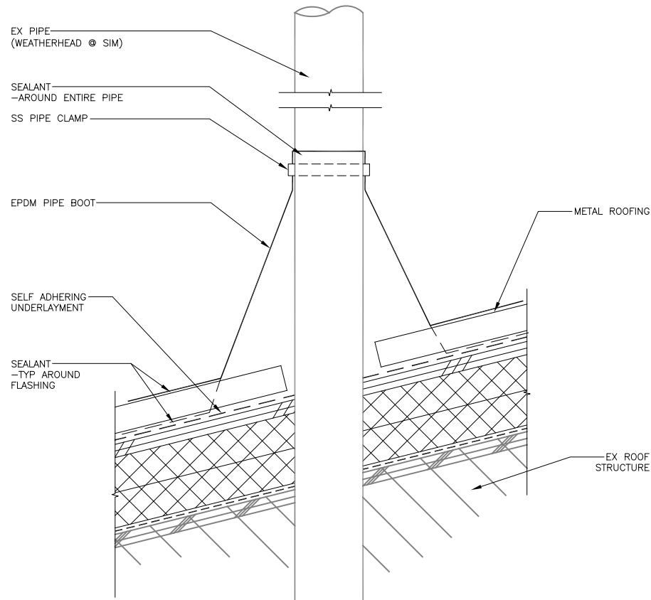
1 TYPICAL ROOF VENT PENETRATION 11086/X_A802-1 SCALE: 0 3" 6" 1'
